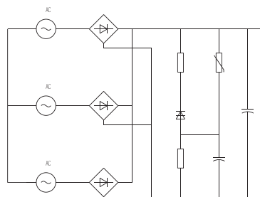
LCDC link with MKP capacitors Pic 2b
