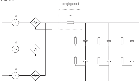
DC link with electrolytic capacitors Pic 2a
